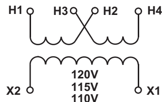
Wiring Diagram
