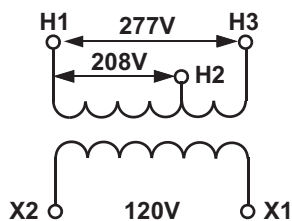
Wiring Diagram
